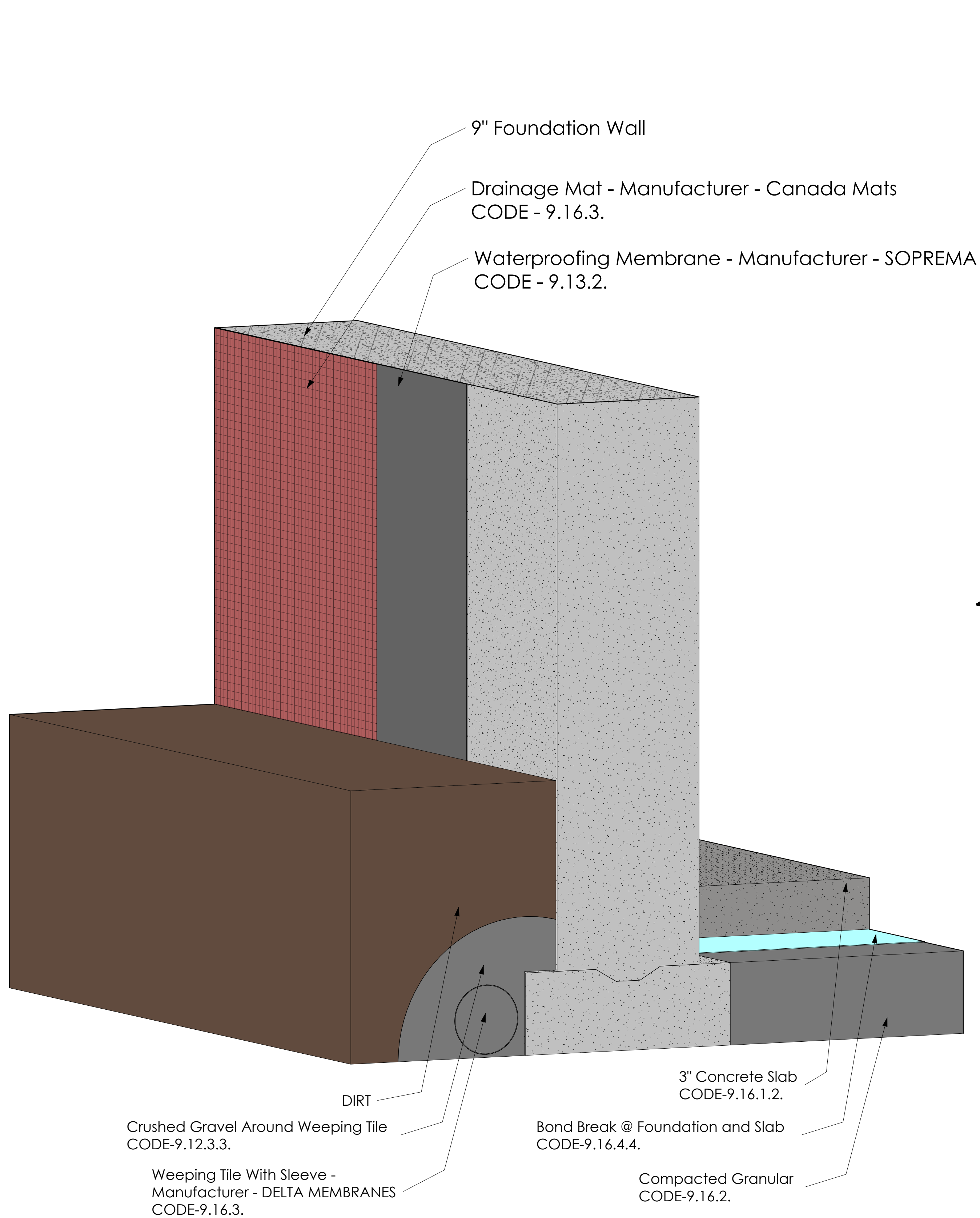
1 3D DETAIL 01 - FOOTING DETAIL
